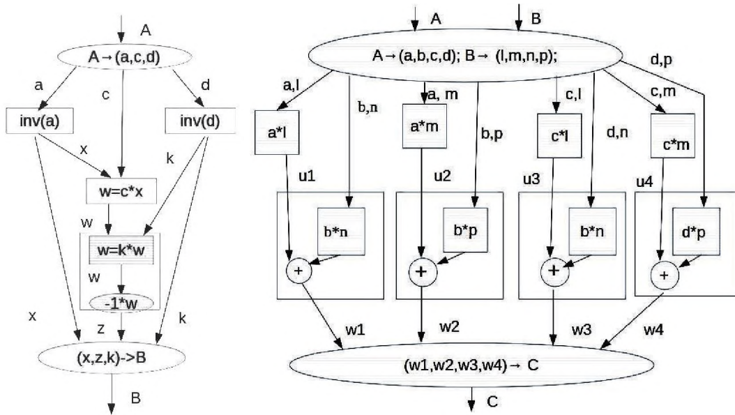
FIGURE 1. The graph of the recursive inversion algorithm of the triangular matrix (on the left) and the graph of the block-recursive matrix multiplication algorithm (on the right).
