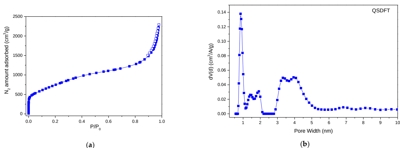
Figure 1. (a). N 2 adsorption (full symbol) and desorption (empty symbol) isotherms at -196\text{ }^{\circ}\text{C} ; (b). Pore size distribution obtained after application of the QSDFT method.
