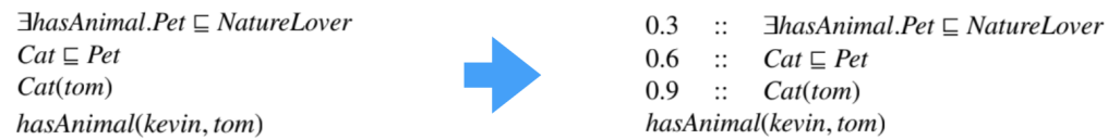
Figure 4. Extension of the logic formalism of description logic \mathcal{ALC} by typicality inclusions.
