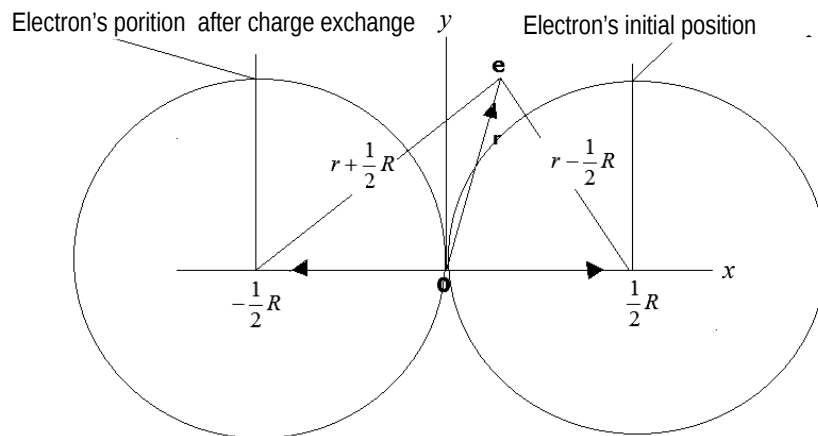
Fig. 3. Position of the electron and its coordinate r
