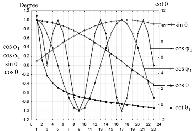
Fig. 5. \sin \theta , \cos \theta , \cot \theta and \cos \varphi for the simulation
