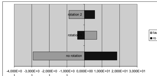
Fig. 10. Gravitational field energy in 2 directions on the spherical curved surface, Case-2 (linear distortion)
