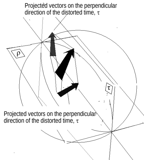
Fig. 11. The Vector projected on tangential (surface) component of the spherical curvature
