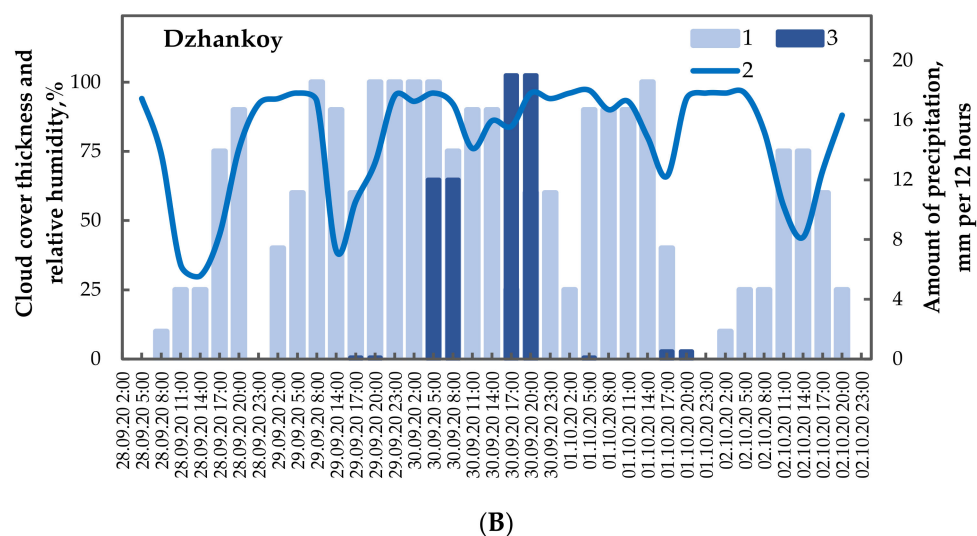
Figure 11. The daily variation in cloud cover thickness (1—scale on the left), relative air humidity (2—scale on the left) and the amount of precipitation (3—scale on the right) at the Simferopol (A) and Dzhankoy (B) meteorological stations for the period from 28 September to 2 October 2020, as a result the passage of the cold front through the Crimean Peninsula and the active influence on atmospheric processes.
