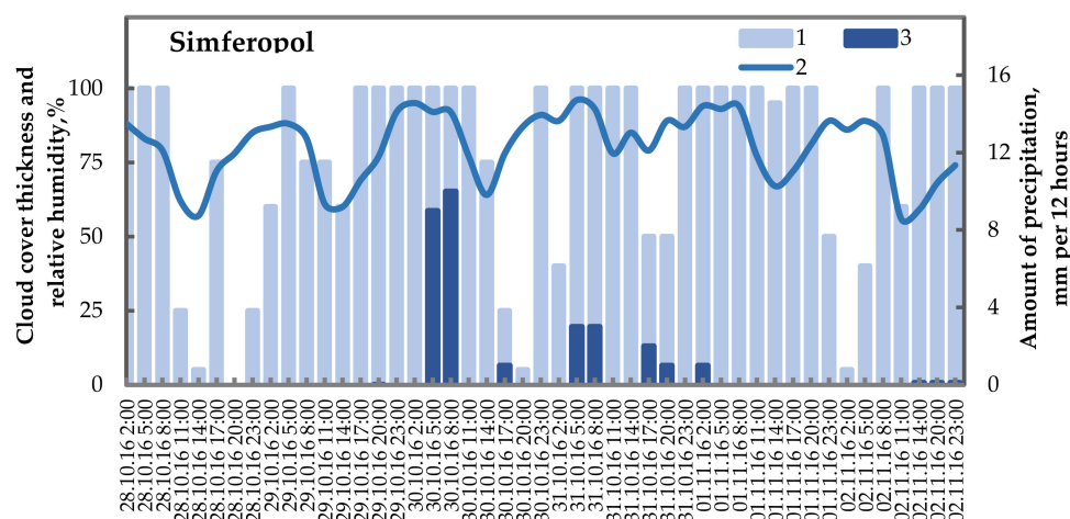
Figure 7. The daily variation in cloud cover thickness (1—scale on the left), relative air humidity (2—scale on the left) and amount of precipitation (3—scale on the right) at the Simferopol meteorological station for the period from 28 October to 2 November 2016, as a result the passage of the cold front through the Crimean Peninsula and the active influence on atmospheric processes.
