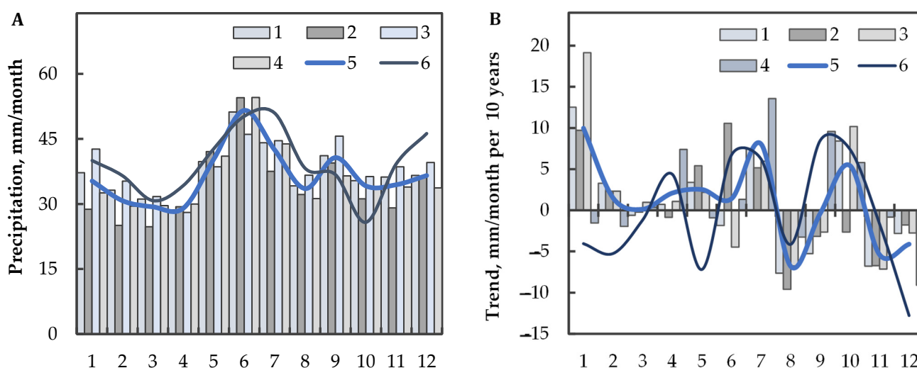
Figure 3. Seasonal variation of precipitation (A) and corresponding trends (B): monthly precipitation values for meteorological stations Zaporizhzhia (1), Mikolaiv (2), Odesa (3), and Kherson (4) as well as for the whole region (5), for the period 1991–2020; 6—values of the climatic norm for the period 1961–1990.
