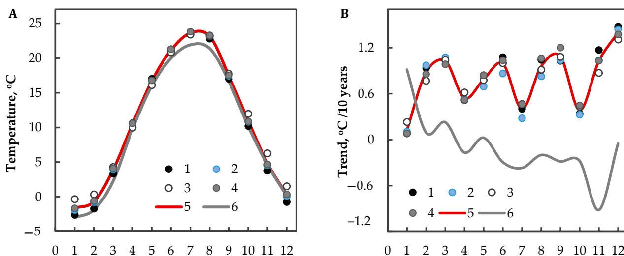
Figure 2. Seasonal variation of temperature (A) and corresponding trends (B): average monthly values for meteorological stations Zaporizhzhia (1), Mikolaiv (2), Odesa (3), and Kherson (4) as well as the values of the climatic norm estimated for the whole region, for the periods 1991–2020 (5) and 1961–1990 (6).
