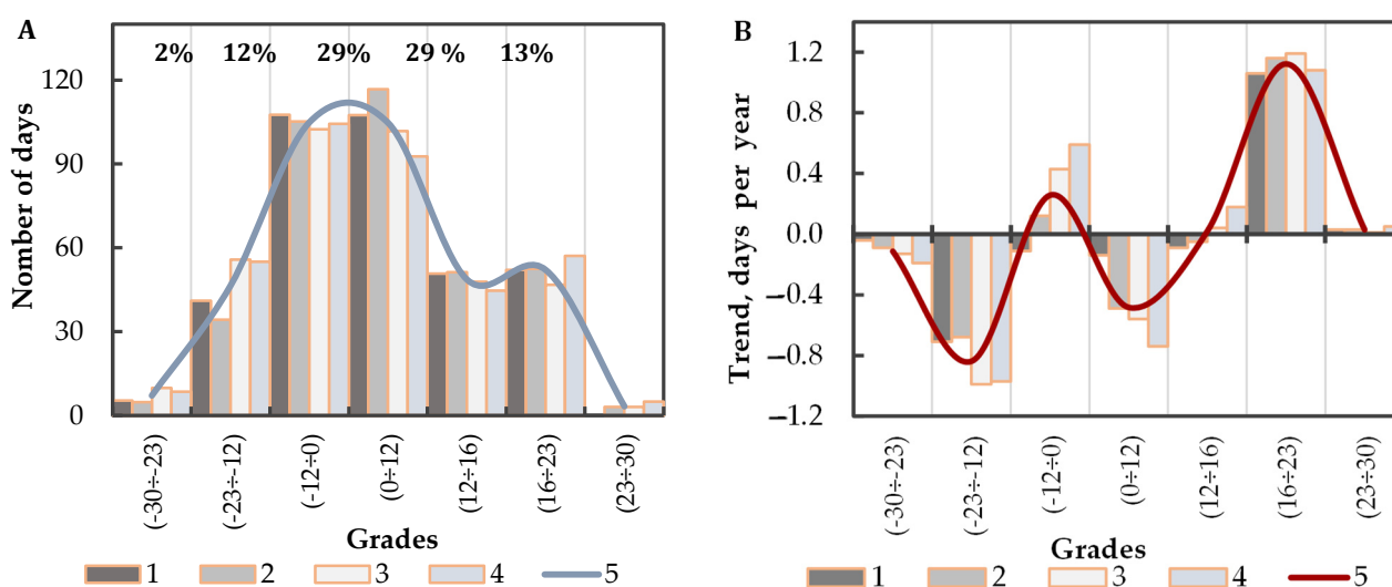
Figure 7. Distribution of the number of days with thermal conditions for humans, due to I_{EET} gradations (A) and corresponding trends (B), based on the data of the meteorostations Zaporizhzhia (1), Mykolaiv (2), Odesa (3), and Kherson (4) as well as for the southern region as a whole (5), for the period 1991–2020.
