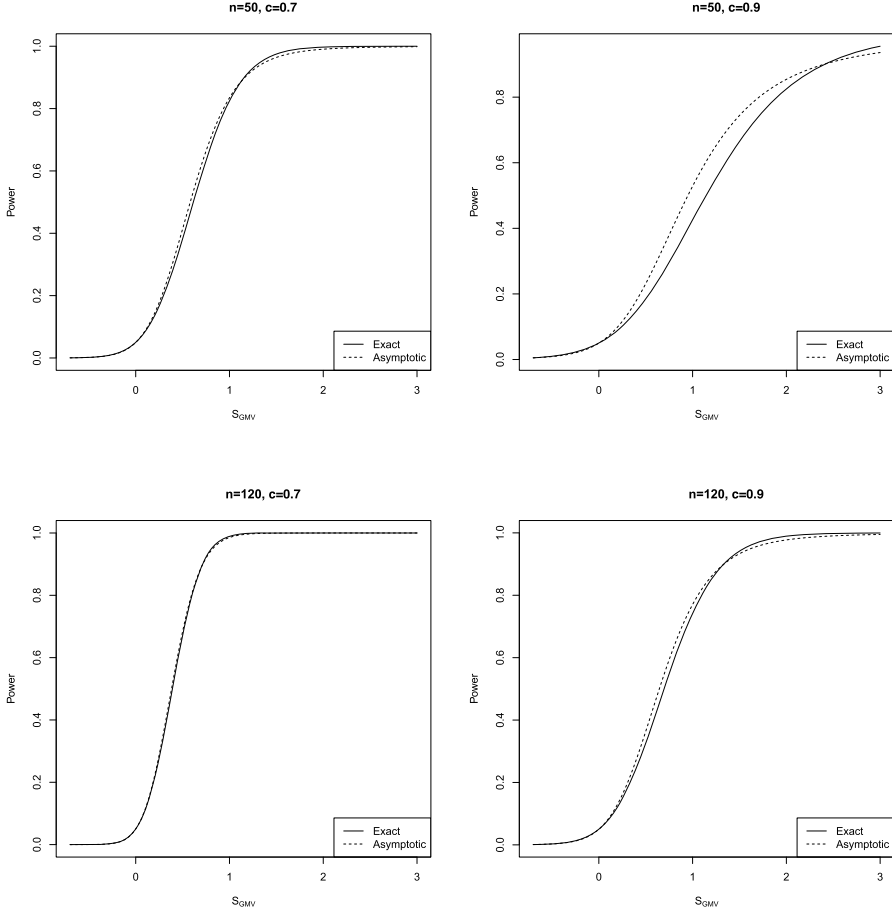
Fig. 3. Powers of the exact test and the high-dimensional asymptotic test as a function of S_{GMV} based on statistic T for n \in \{50, 120\} and c \in \{0.7, 0.9\} with s = 1 and \alpha = 5\%
