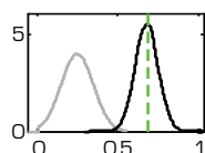
Fig. 1. Prior and posterior densities of \phi
